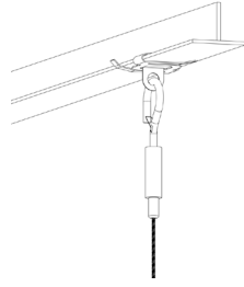
T-Bar Clip and Clevis Hook
